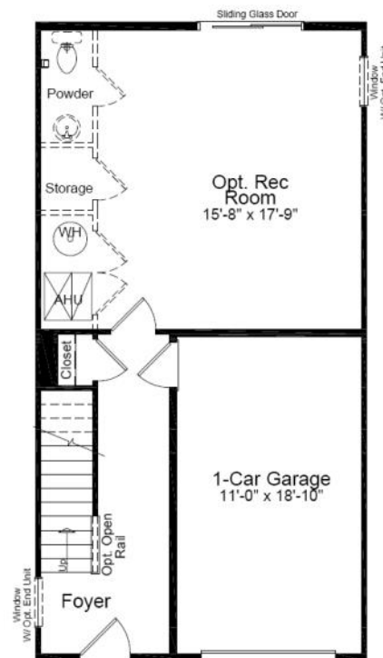
Lower Level Floorplan with Opt. Extension
