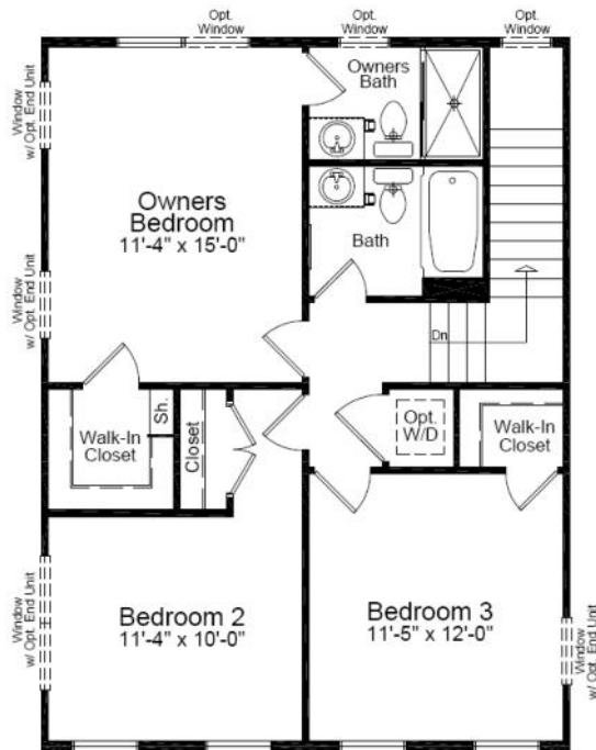
Upper Level Floorplan
