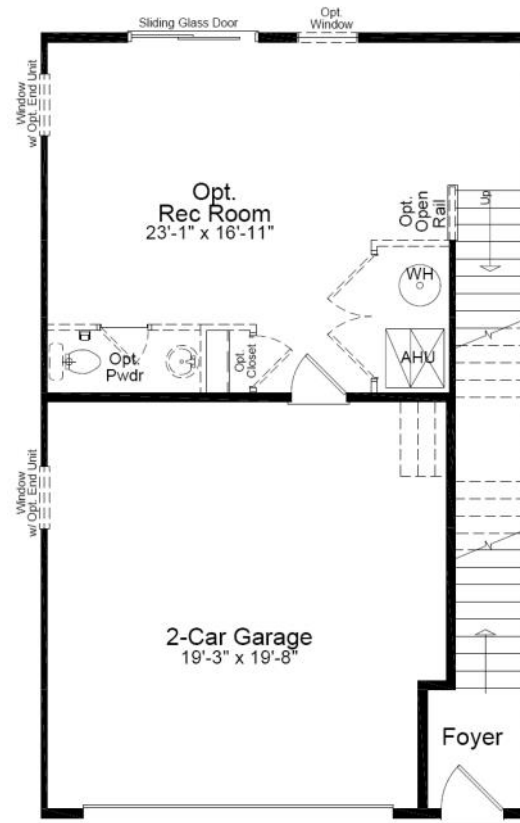
Lower Level Floorplan with Opt. Extension
