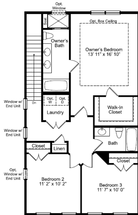
Upper Level Floorplan with Opt. Extension
