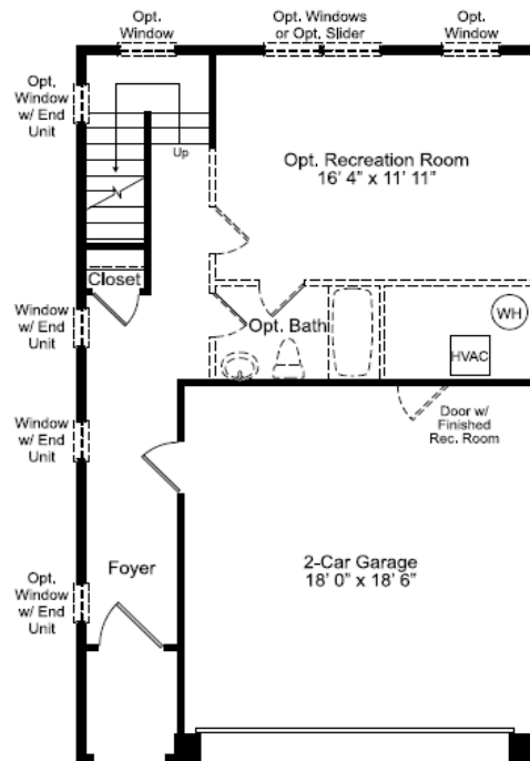
Lower Level Floorplan
