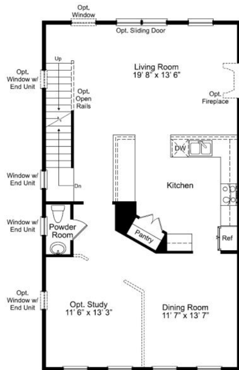
Main Level Floorplan with Opt. Extension
